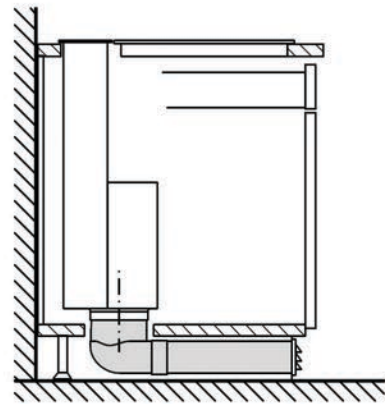
B: Exterior wall – U-value > 0.5 \text{ W}/(\text{m}^2\text{K})
