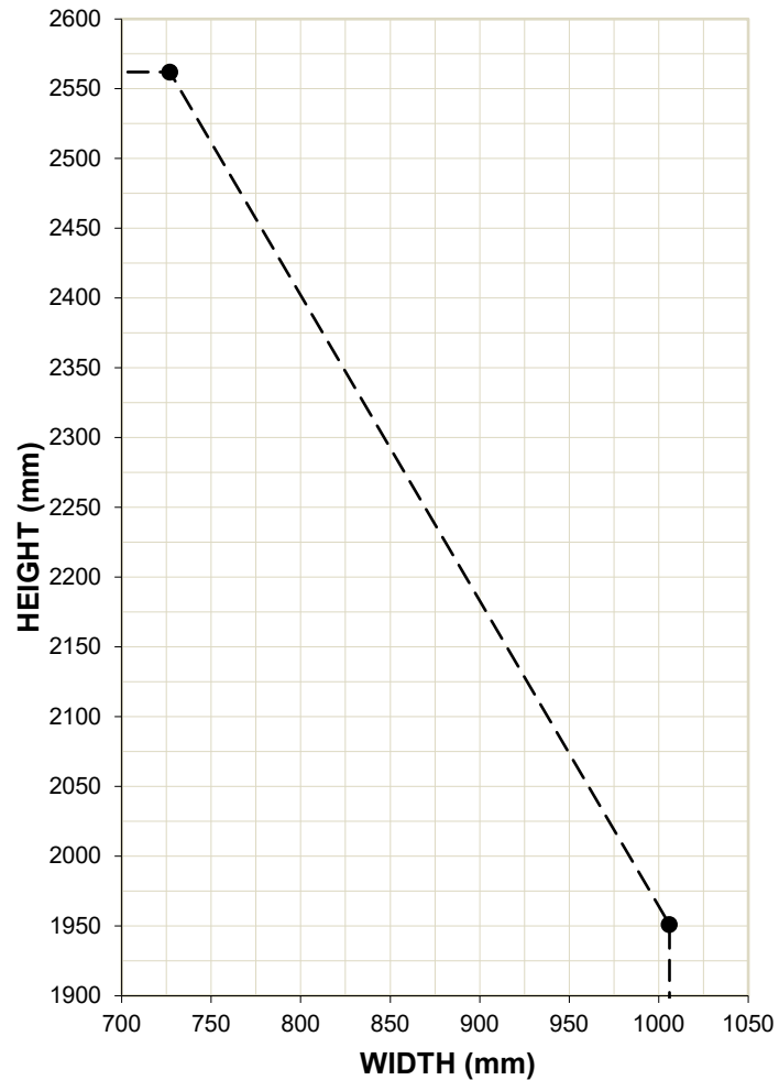
FIGURE A01 FD30 LATCHED SINGLE DOOR ASSEMBLIES
