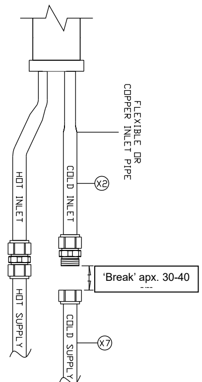
Example tap connections after the 'break' is created:
