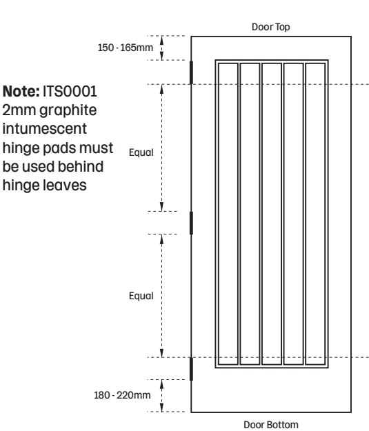
Diagram 1 - Hinge Positions
