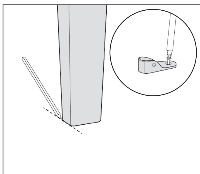
19 Mark position on the floor. Remove the support and fix the bracket to the floor using suitable fixings (not supplied).
