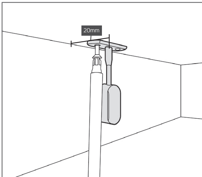
11 Place the centre of the hanger bar bracket at the measure line and screw into place.
