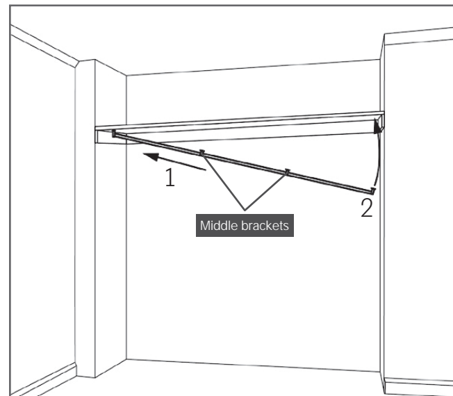
12 1. Thread the middle two brackets. 2. Fix the opposite end bracket in place. Evenly space the middle brackets and fix in position.
